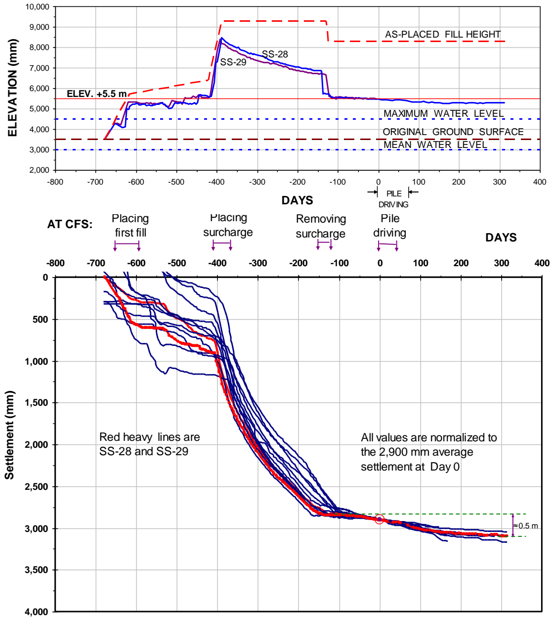
Fig. 8 Fill and surcharge elevation and ground surface settlement
