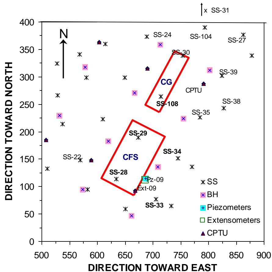
Fig. 6 Locations of CFS and CG buildings and layout of field instrumentation
