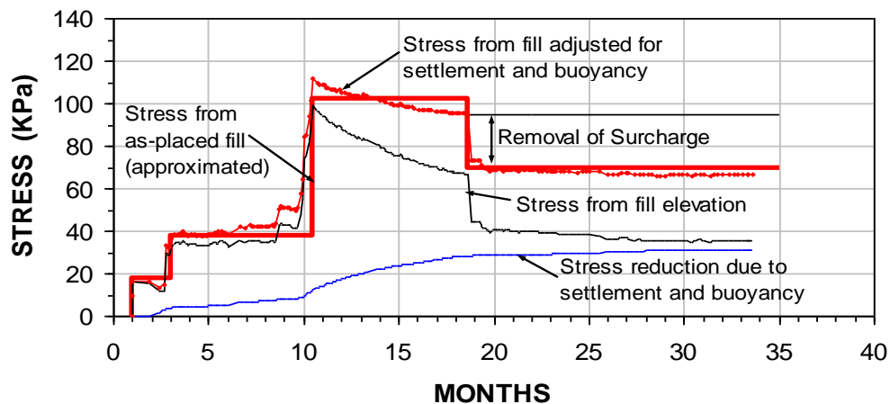
Fig. 13 Actual loading and unloading stresses
