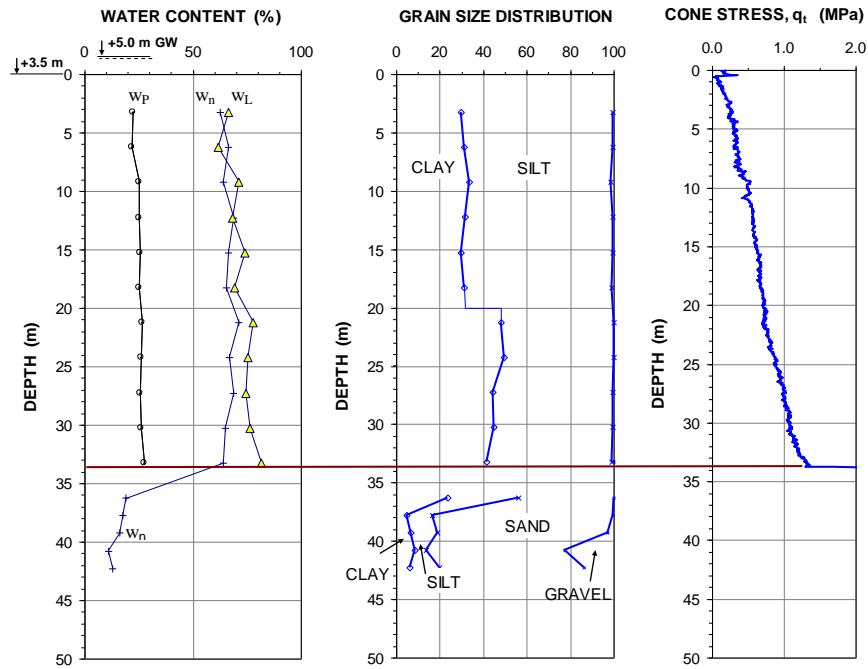
Fig. 2 Consistency limits, grain size distribution, and CPTU cone stress
