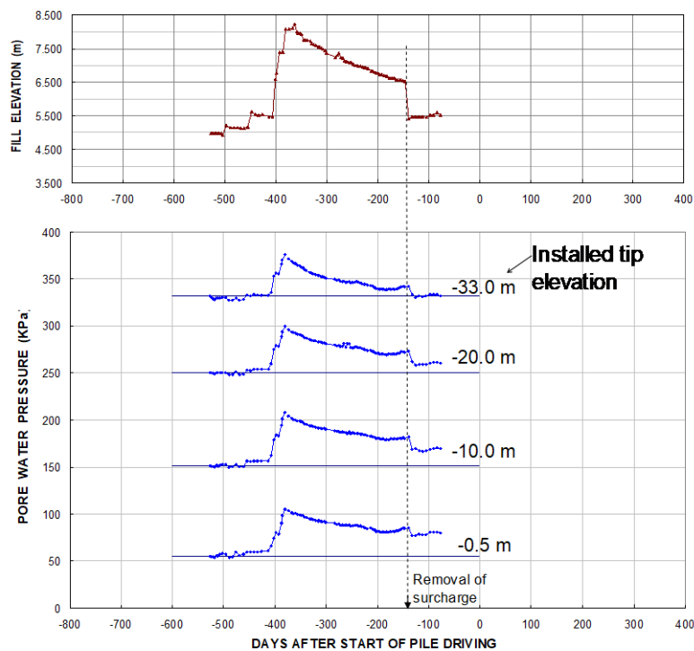
Fig. 10 Fill height and pore pressures measured between Days -527 and -77 at the CFS building
