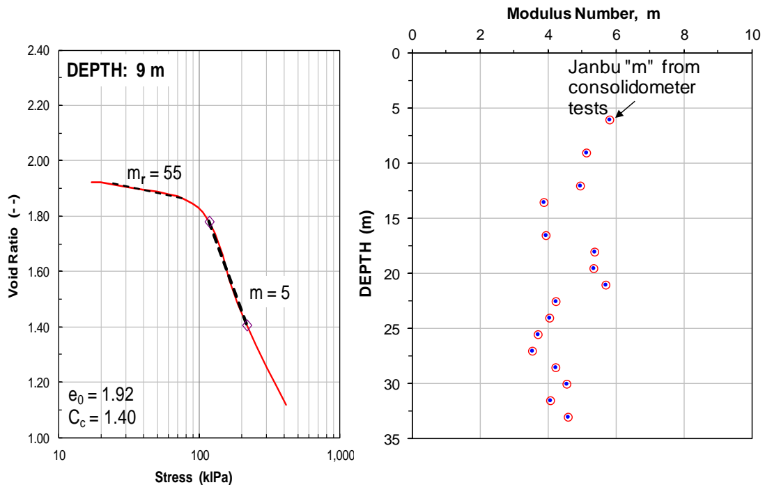
Fig. 3 Typical results of a consolidometer test and distribution of modulus number determined from consolidometer tests and from CPTU cone stress. The depth scale is from original ground surface; Elev. +3.5 m.
