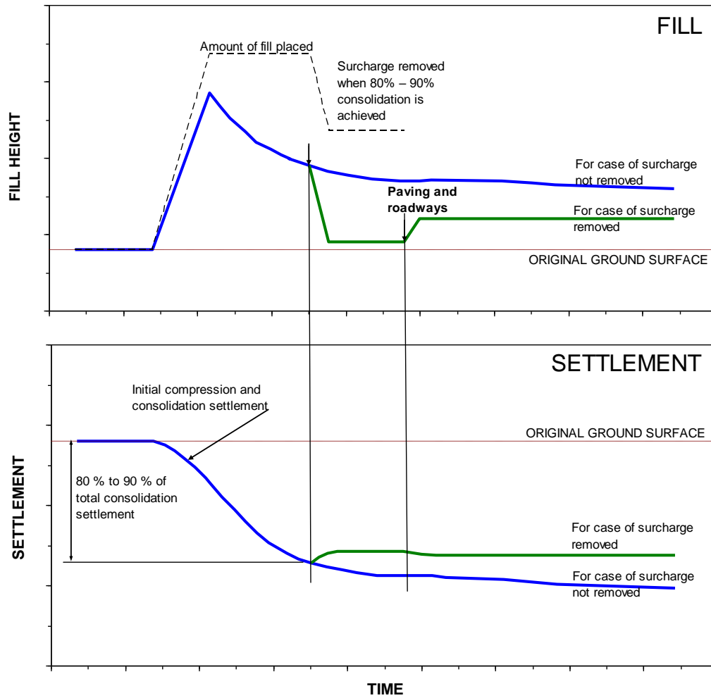
Fig. 4 Principles of wick drain and preloading site improvement work
