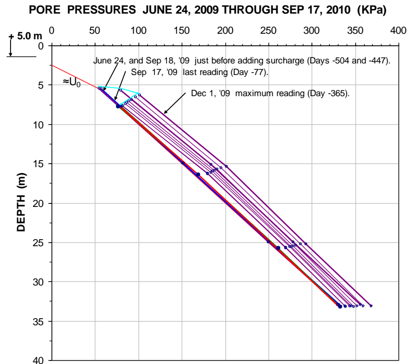
Fig. 11 Pore pressures versus depth
