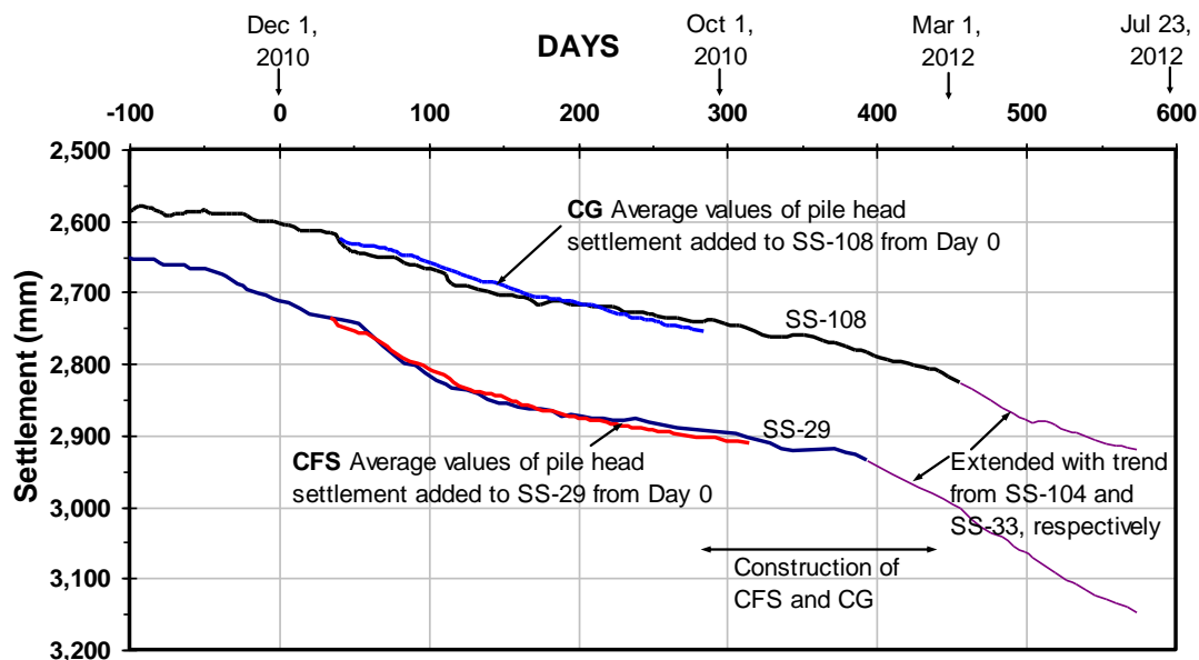
Fig. 16. Settlements measured at the SS-plates near the respective building and settlement of the piles before lengthening
