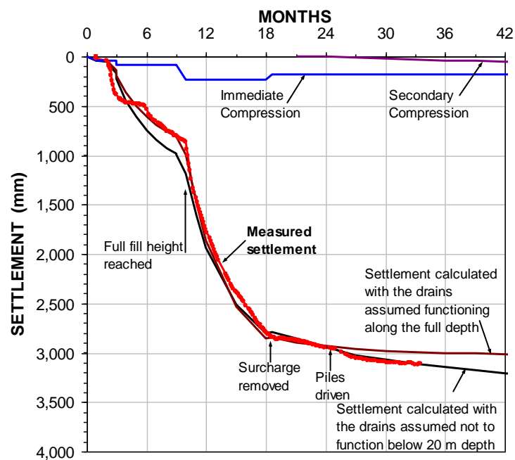
Fig. 14 Results of back-analyses to fit measured settlements
