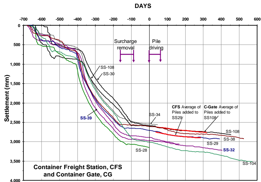
Fig. 7 Ground surface and pile settlements
