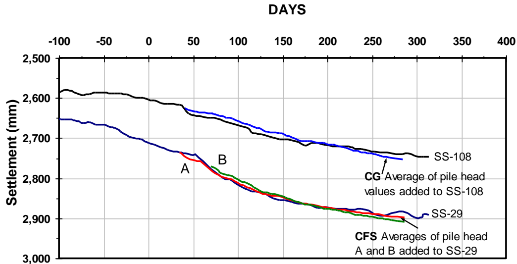
Fig. 12 Settlements of SS-29 and SS-108 located within the footprint of the buildings and the average settlement of the pile heads from end of driving.
