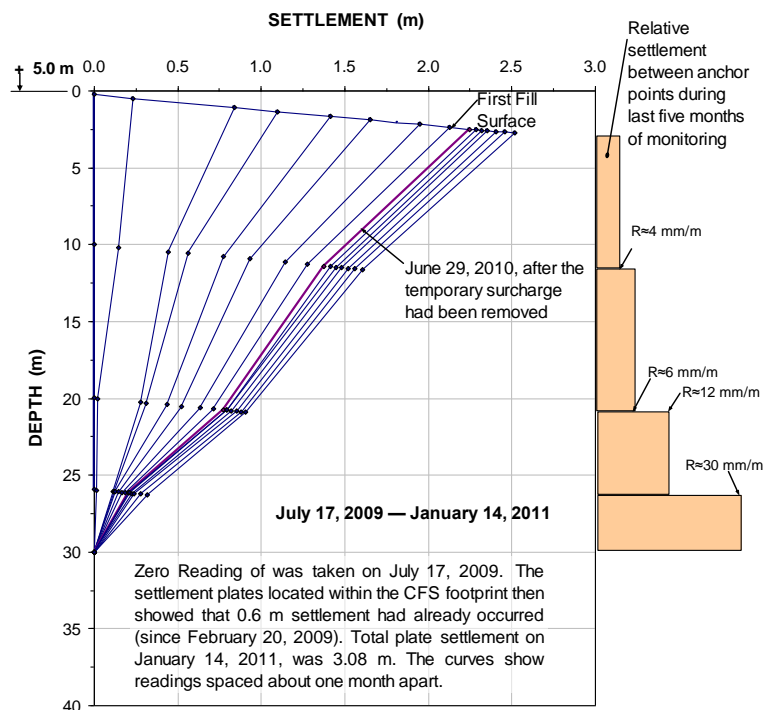
Fig. 9 Distribution of settlement with depth
